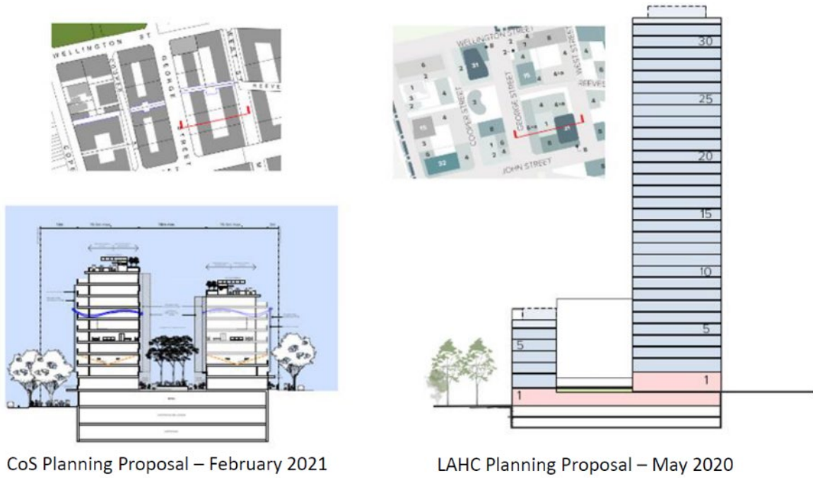
Figure 39 Comparative section through site
