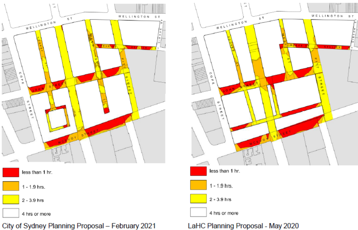
Figure 40 Comparison of sunlight to streets in mid-winter
